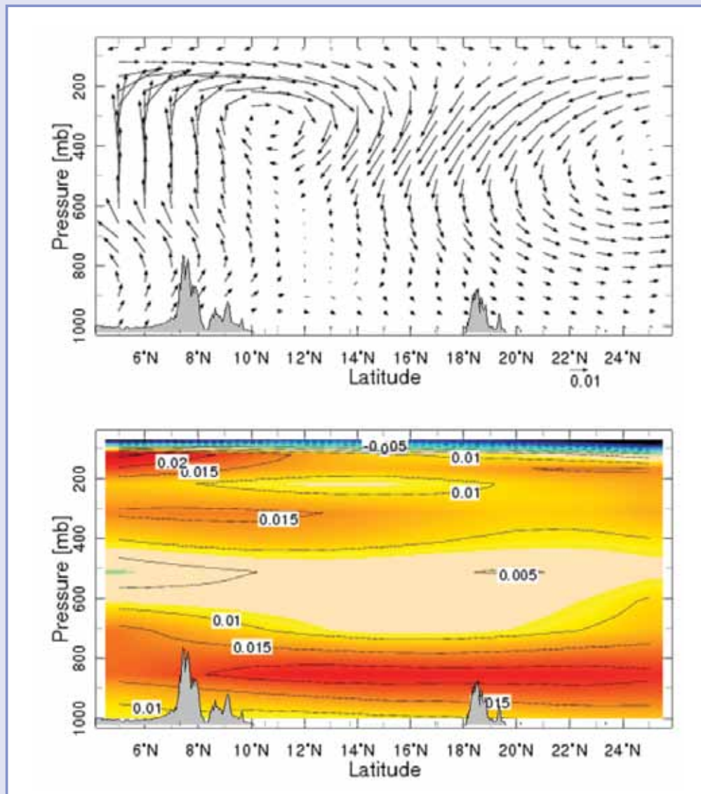
Figure 24: The analysis is of linear trends in the meridional atmospheric Hadley circulation (top, m/s /yr) and air temperature (C/yr), as N-S height sections across Puerto Rico from NCEP reanalysis 1948-2009. Adapted and updated from Jury and Winter (2009).
