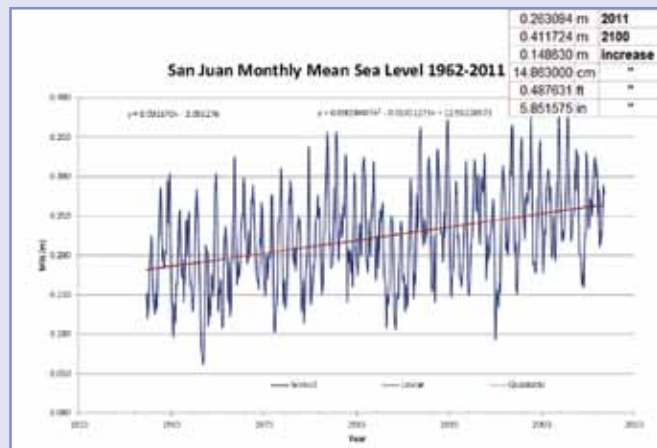
Figure 47: Tide gauge data from San Juan show that from 1962 to 2011 the North Coast of Puerto Rico experienced a 1.65 mm/yr rise in sea level. From 2001 to 011 the rise was 0.50 mm/yr. Source: Dr. Jorge Capella 2011, UPR/CariCOOS.
