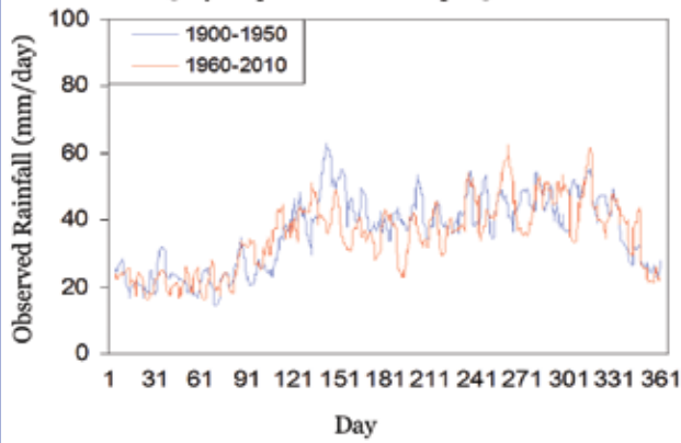
Figure 36: Daily rainfall averaged over annual cycle in two 50yr periods using data combined from Mayaguez, Manati and Manuabo for top 2.5% of cases. Notice the decrease in May floods (days 121-151).
