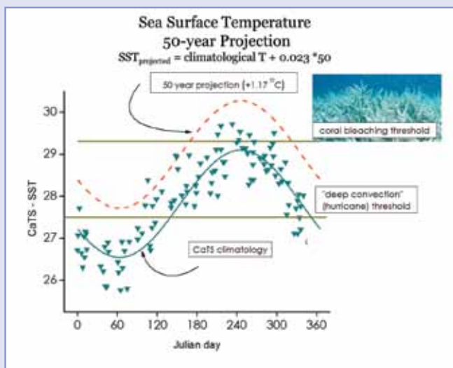
Figure 43: OI v2 SST trend ( 0.023^{\circ}\text{C}/\text{yr} ) and climatology obtained at the Caribbean Time Series Station ( 17^{\circ}36' \text{N } 67^{\circ}\text{W} ; 1994 – 2007 monthly data). An increase of 1.17^{\circ}\text{C} ( 2.1^{\circ}\text{F} ) over a 50 year period can be expected.
